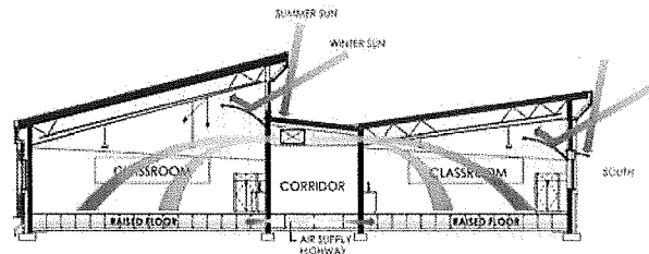
Fig. 4: Typical classroom section
