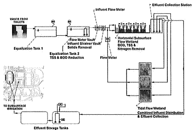
Fig. 3: Living Machine flow diagram
