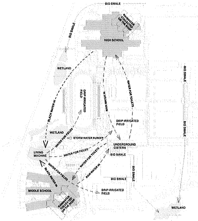
Fig. 1: Overall water cycle
