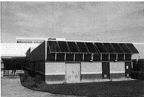
Fig. 10 Solar hot water system
