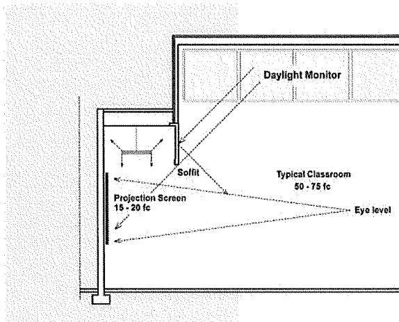
Fig. 7 Architectural shading strategy
