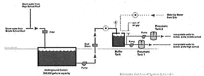
Fig. 2: Rainwater collection flow diagram
