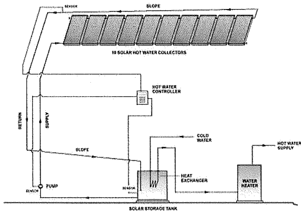
Fig. 9 Solar hot water schematic diagram
