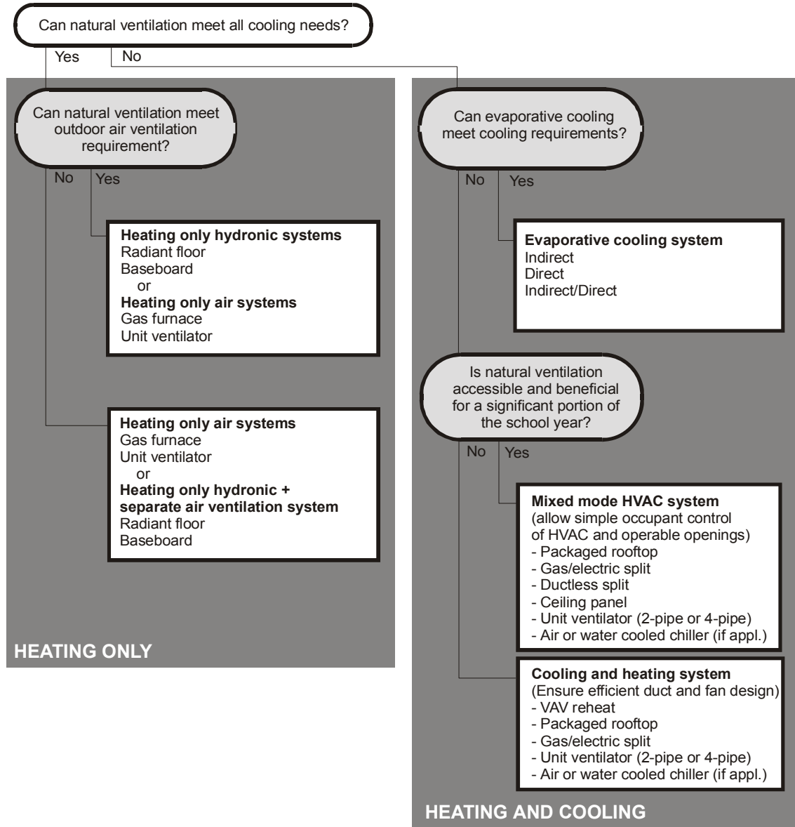
Figure 34 – HVAC System Selection Decision Tree
