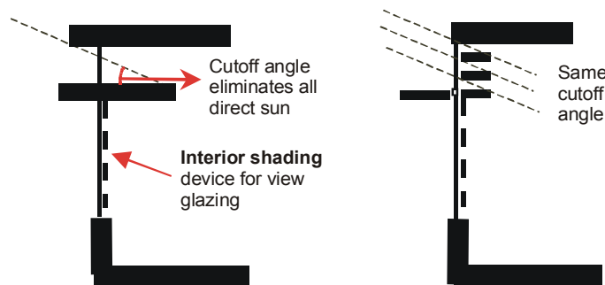
Figure 6 – Cutoff Angle of Light Shelves
