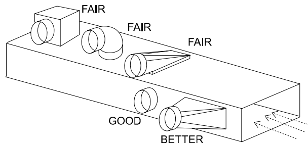
Figure 36 – Various Connections for Branch Ducts
