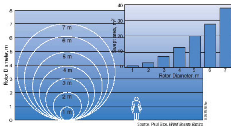
Figure 40 – Relative Size of Small Wind Turbines
