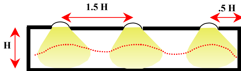
Figure 8 – Skylight Grid Spacing
