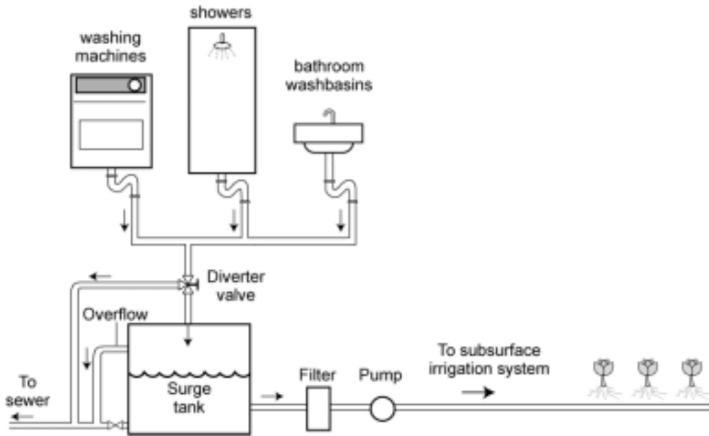
Figure 48 – Example Schematic of Gray Water System
