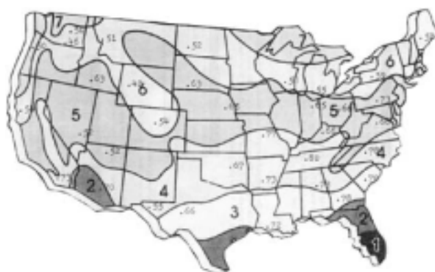
Figure 39 – Solar Insolation Levels in the United States
