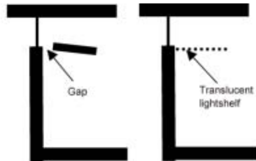
Figure 7 – Creating a Wall Wash
