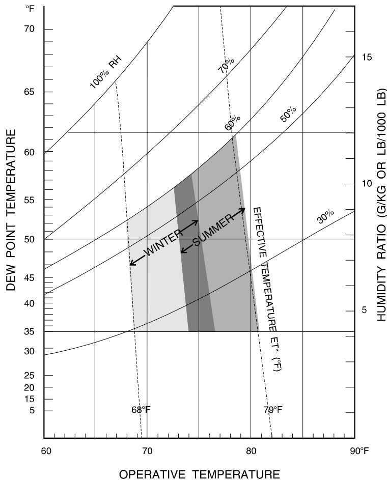
Figure 26 – ASHRAE Standard 55 Comfort Envelope
