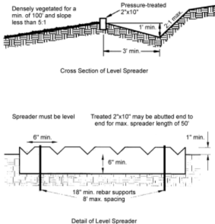
Figure 46 – Level Spreader, Cross Section & Detail
