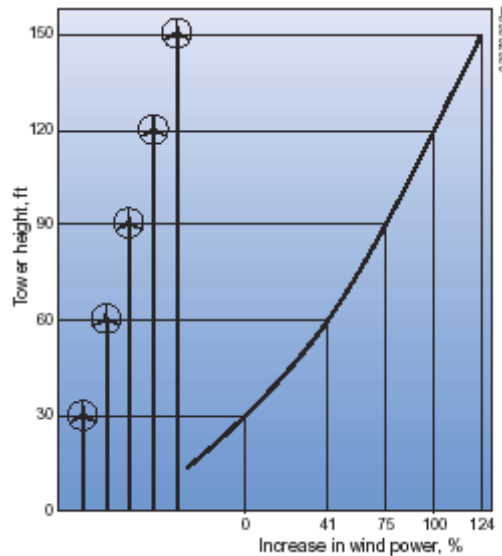
Figure 41 – Wind Speeds Increase with Height
