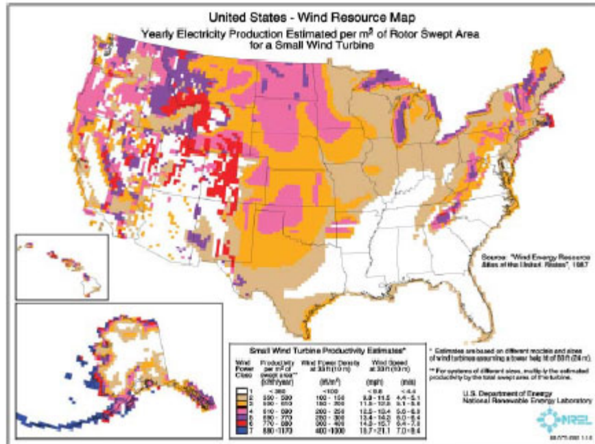
Figure 43 – Wind Resource Map
