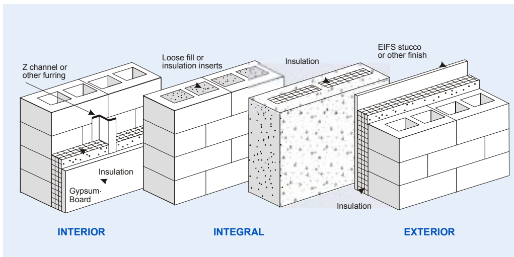
Figure 12 – Mass Wall Constructions
