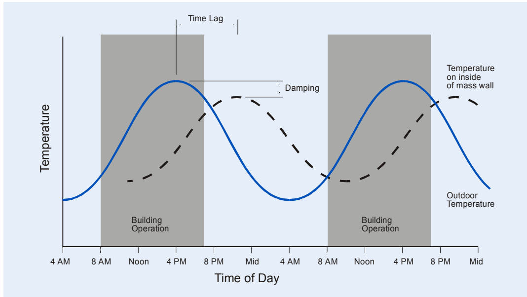
Figure 11 – Temperature Swing
