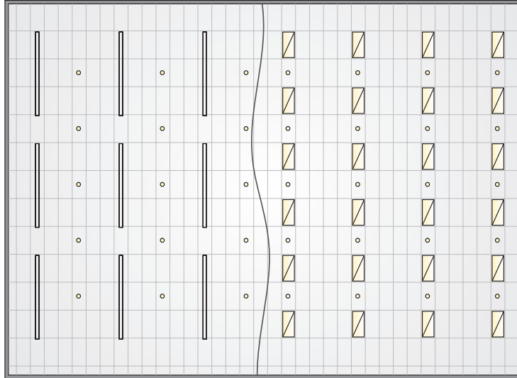
Figure 24 – Multipurpose Lighting Designs
