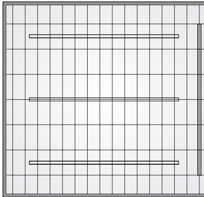
Figure 21 – Industrial Classroom Suspended Lighting Design
