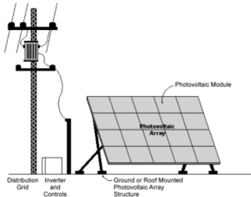
Figure 45 – PV Siting, Elevated
