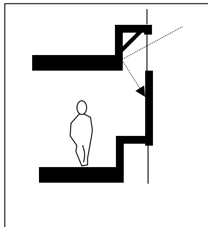
Figure 5 – Clerestories in Multistory Buildings
