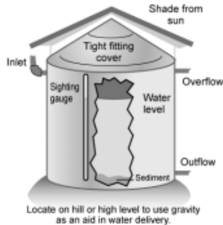
Figure 47 – Cistern for Rainwater Collection
