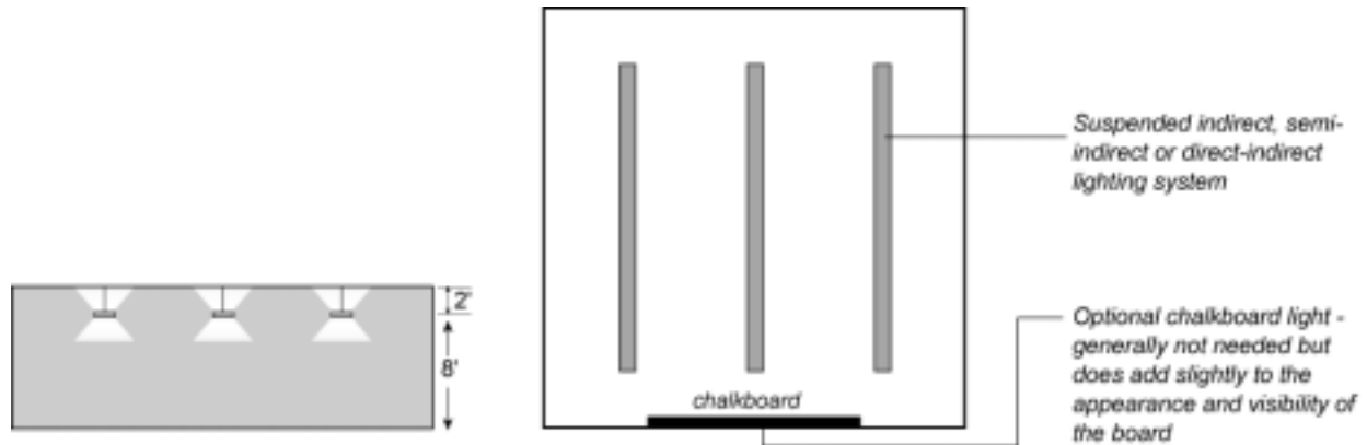
Figure 19 – Classroom Pendant-Mounted Lighting Design
