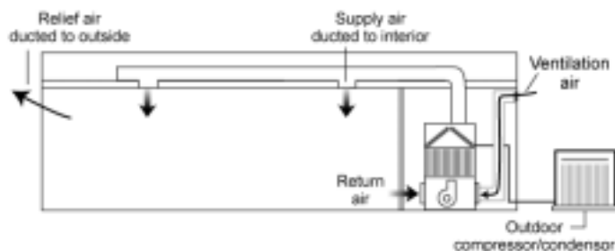
Basic gas/electric split system.
