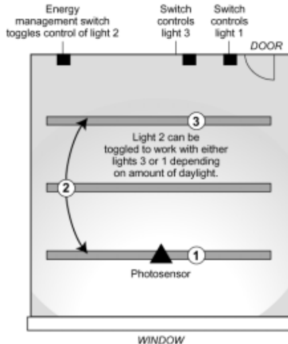
Figure 22 – Simple Windowed Classroom Control
