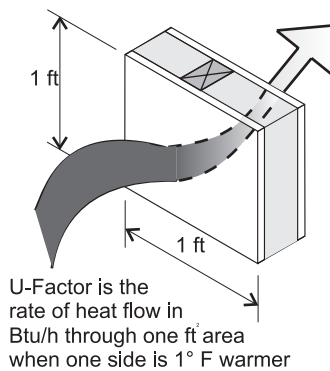
Figure 10 – Concept of U-factor
