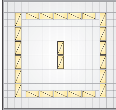
Figure 20 – “Modified Doughnut” Classroom Recessed Lighting Design
