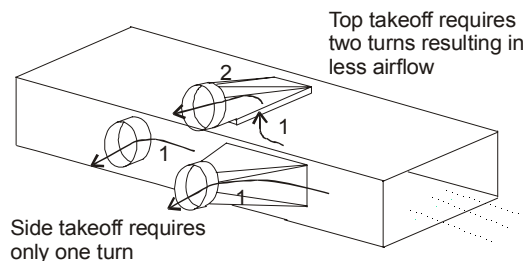
Figure 37 – Side Takeoff Vs. Top Takeoff
