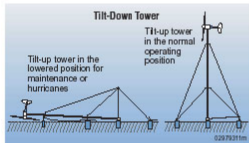
Figure 42 – Tilt-Down Towers
